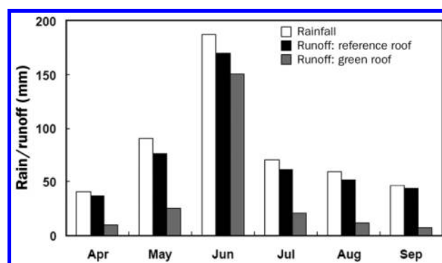
Figure 4. Storm-water runoff retention in a green-roof test plot in Ottawa, Ontario, Canada, in 2002. Values are sums of total runoff retained. The green roof had 15 centimeters of growing medium and was planted with lawn grasses (Liu and Baskaran 2003); it was compared with an adjacent conventional roof of the same size.
