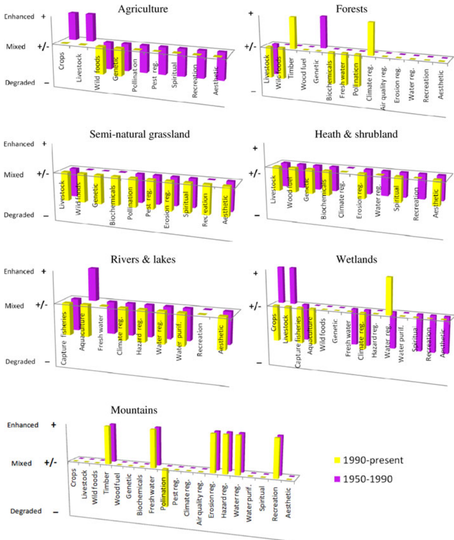
Fig. 2 Trends in the status of European ecosystem services. Enhancement refers to increases in production area or amount, or a change in service which leads to greater benefits for people, while degradation refers to current use exceeding sustainable levels or a reduction in the benefits for people either through a change in the service or through human pressures on the service exceeding its limits (MA 2005a). Mixed refers to mixed trend across Europe
