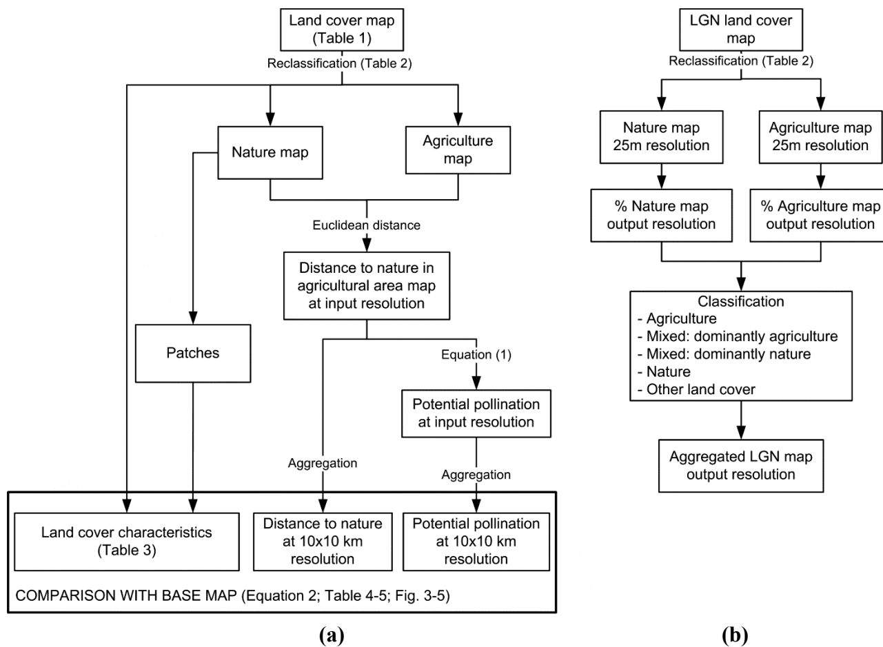
Figure 1. (a) Flowchart of the analyses; and (b) Procedure for aggregating the 25-m resolution Land Use Map of the Netherlands (LGN).
